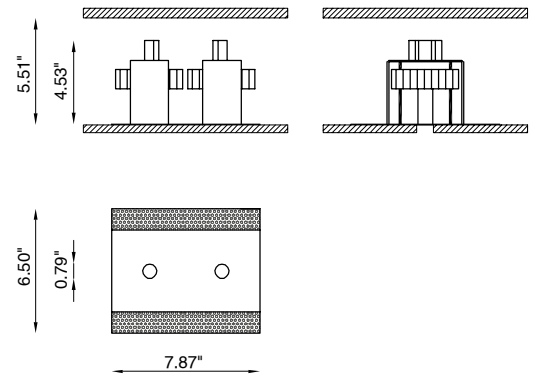
Fixture Dimensions
