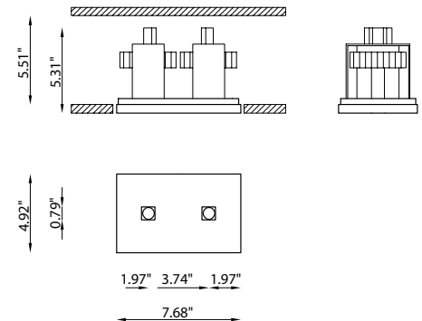
Fixture Dimensions
