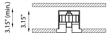
Ceiling Cut-Out: 3.94" x 3.94" Fixture Dimensions:
