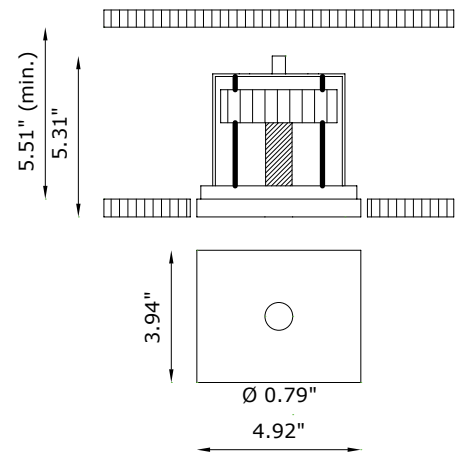
Ceiling Cut-Out: 5.31" x 4.33" Fixture Dimensions:
