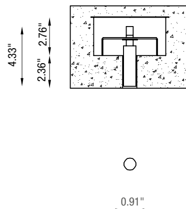
Fixture Dimensions:
