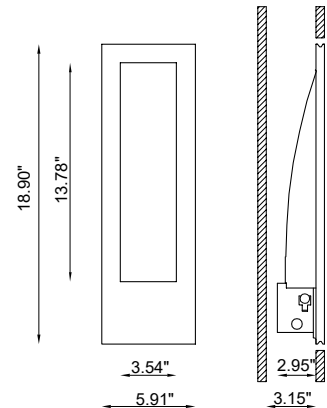
Fixture Dimensions
