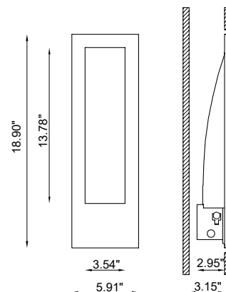
Fixture Dimensions
