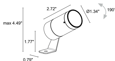
Fixture Dimensions
