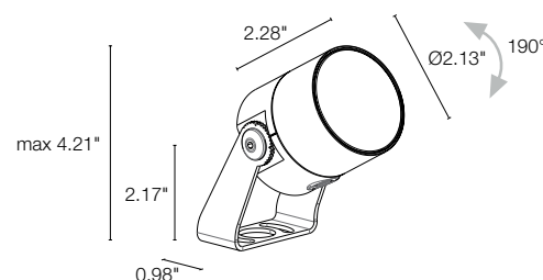
Fixture Dimensions
