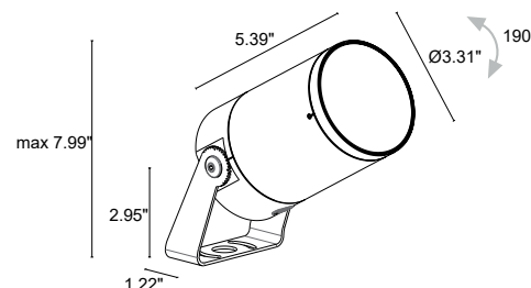
Fixture Dimensions
