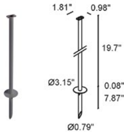
WP1006__ (Length 19.69") WP1007__ (Length 31.50") Ground Spike with Bracket Include one of the below finishes:
