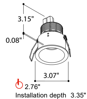
Fixture Dimensions
