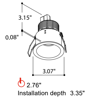
Fixture Dimensions
