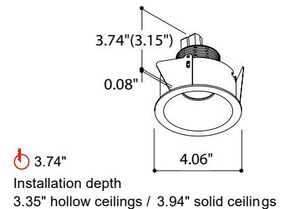
Fixture Dimensions
