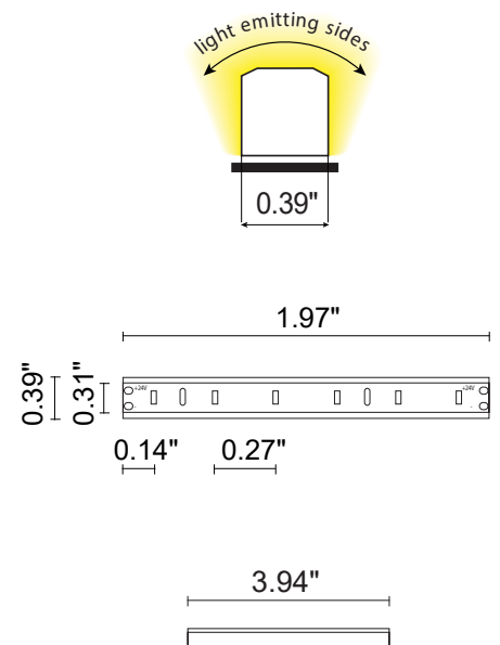
Fixture Dimensions
