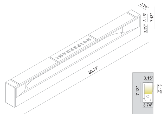
Ceiling Cut-Out: 50.98" x 7.32" Fixture Dimensions
