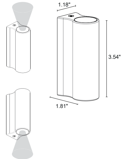
Fixture Dimensions
