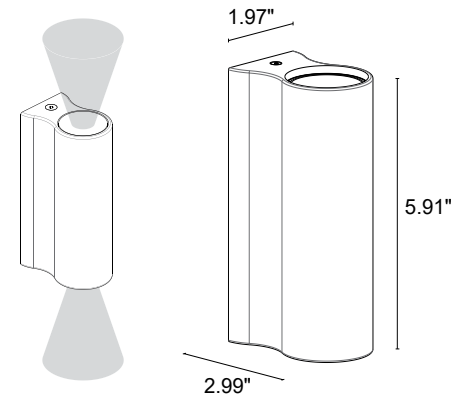
Fixture Dimensions
