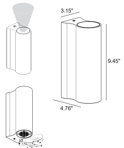
Fixture Dimensions
