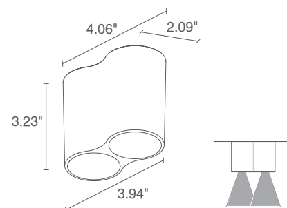
Fixture Dimensions
