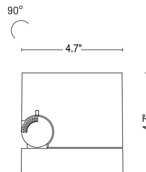
Fixture Dimensions
