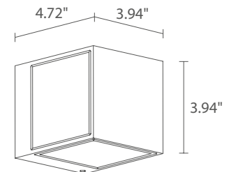
Fixture Dimensions
