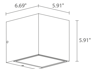
Fixture Dimensions
