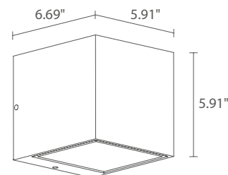
Fixture Dimensions
