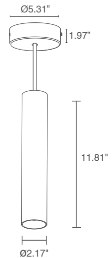
Fixture Dimensions
