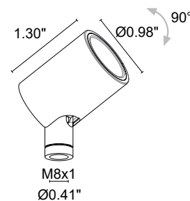
Fixture Dimensions
