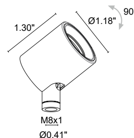
Fixture Dimensions
