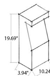
Fixture Dimensions
