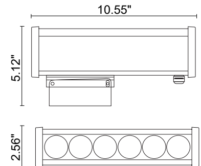
Fixture Dimensions
