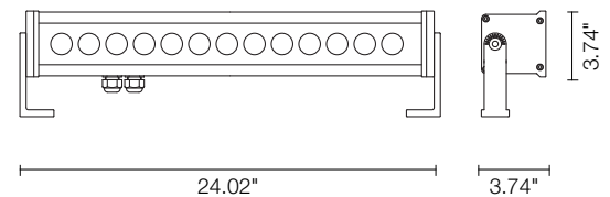
Fixture Dimensions
