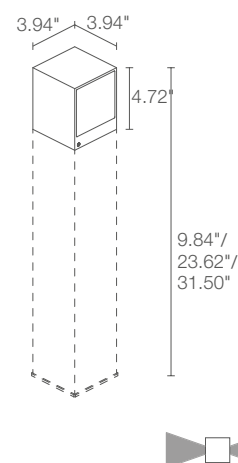
Fixture Dimensions
