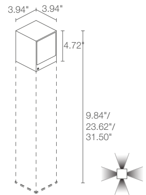
Fixture Dimensions
