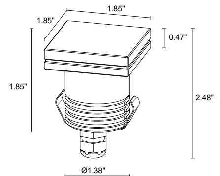
Fixture Dimensions
