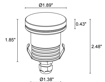
Fixture Dimensions
