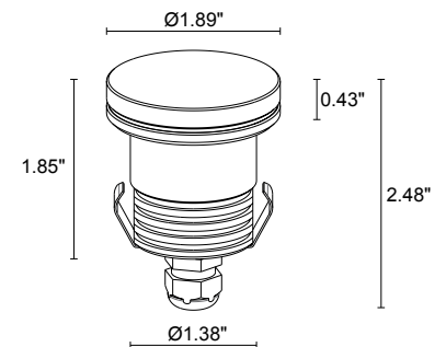
Fixture Dimensions
