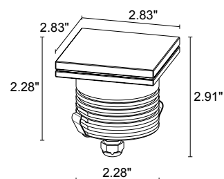
Fixture Dimensions
