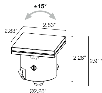
Fixture Dimensions
