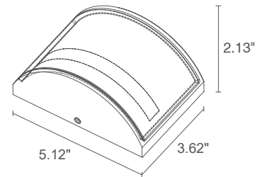
Fixture Dimensions
