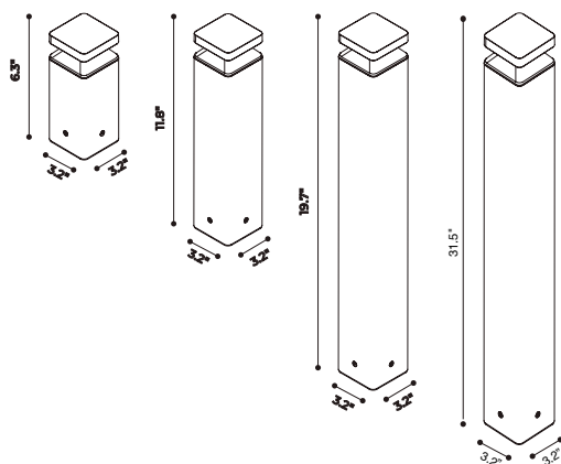
Fixture Dimensions
