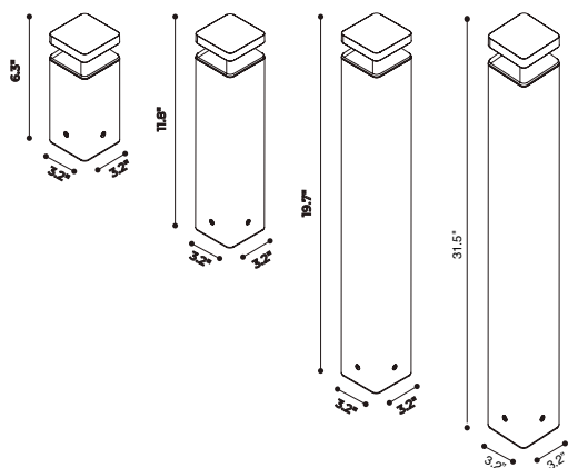
Fixture Dimensions
