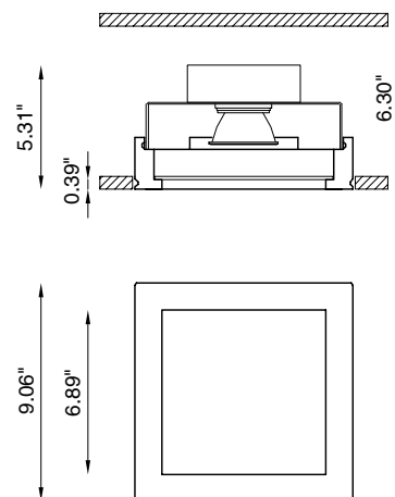
Fixture Dimensions
