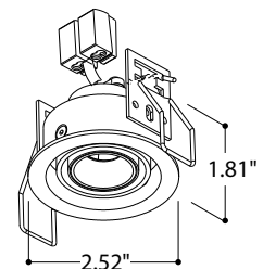
Fixture Dimensions
