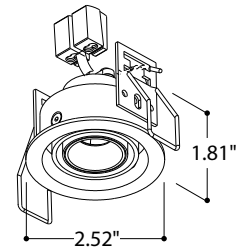
Fixture Dimensions
