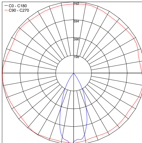
PHOTOMETRIC FILENAME : MICRO HELAX DIMWARM.IES
