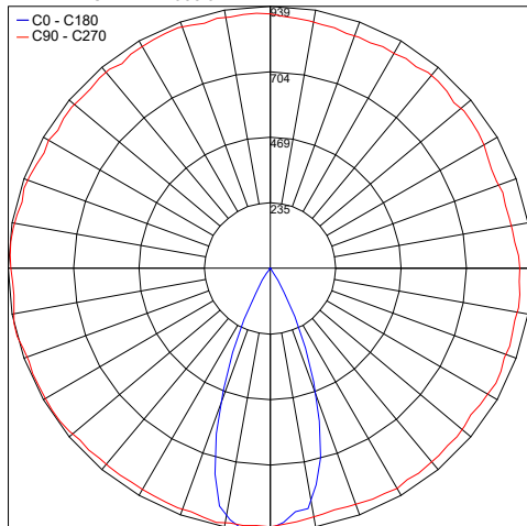
PHOTOMETRIC FILENAME : MICRO HELAX 2700K BEAM 36°.IES
