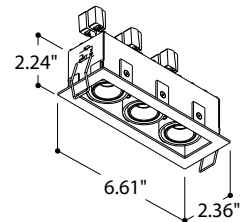
Fixture Dimensions
