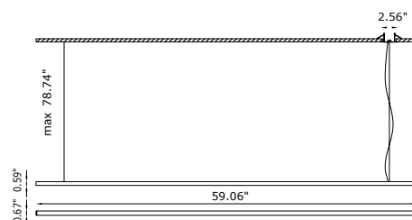
Fixture Dimensions
