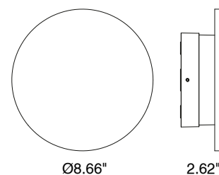
Fixture Dimensions
