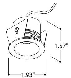
Fixture Dimensions
