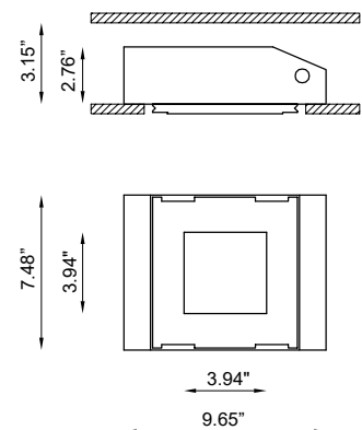
Fixture Dimensions
