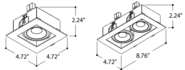
Fixture Dimensions
